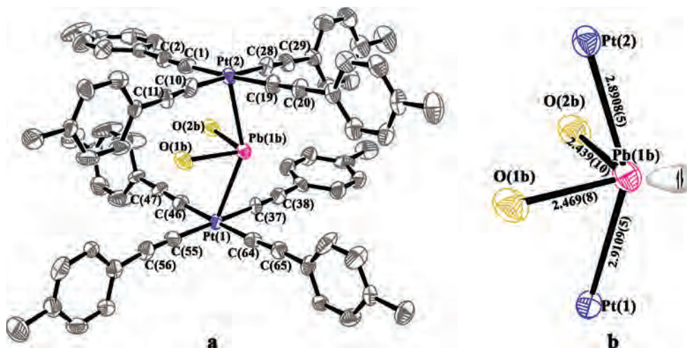
Figure 1. (a) Molecular structure of the major component in the positional disorder showed by the anion [\{\text{Pt}(\text{C}\equiv\text{CTol})_4\}_2\text{Pb}(\text{OH}_2)_2]^{2-} in 1 (major component). Ellipsoids are drawn at 50% probability level and hydrogen atoms omitted for clarity. (b) Hemidirected trigonal bipyramid coordination around the lead center, showing the presumed location for the lone pair.
