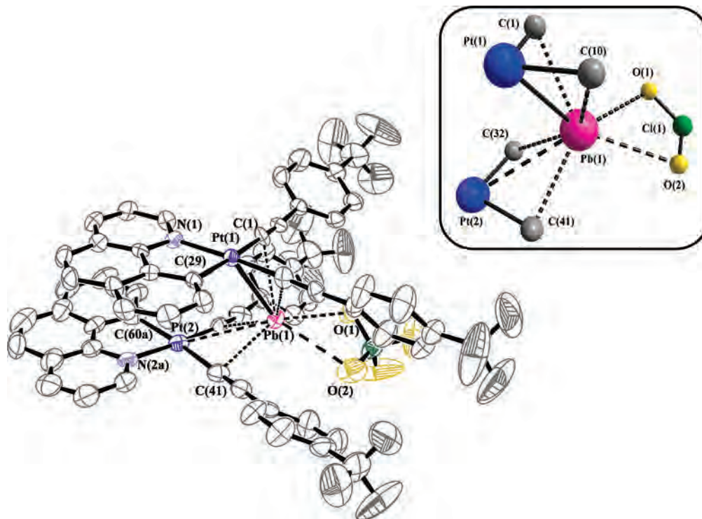
Figure 3. Molecular structure of the adduct anion [\{Pt(bzq)(C\equiv CC_6H_4-CF_3-4)_2\}_2Pb(O_2ClO_2)]^- in 4 , with the coordination around the Pb^{II} in the inset. Ellipsoids are drawn at 50% probability level. Hydrogen atoms are omitted for clarity.
