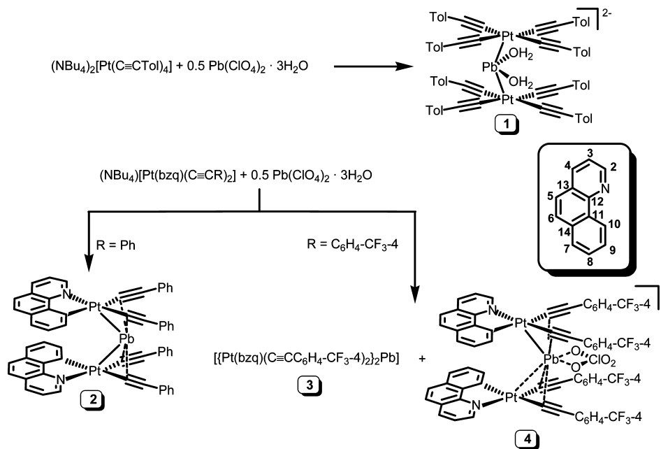
Figure 3. Molecular structure of the adduct anion [\{Pt(bzq)(C\equiv CC_6H_4-CF_3-4)_2\}_2Pb(O_2ClO_2)]^- in 4 , with the coordination around the Pb^{II} in the inset. Ellipsoids are drawn at 50% probability level. Hydrogen atoms are omitted for clarity.
